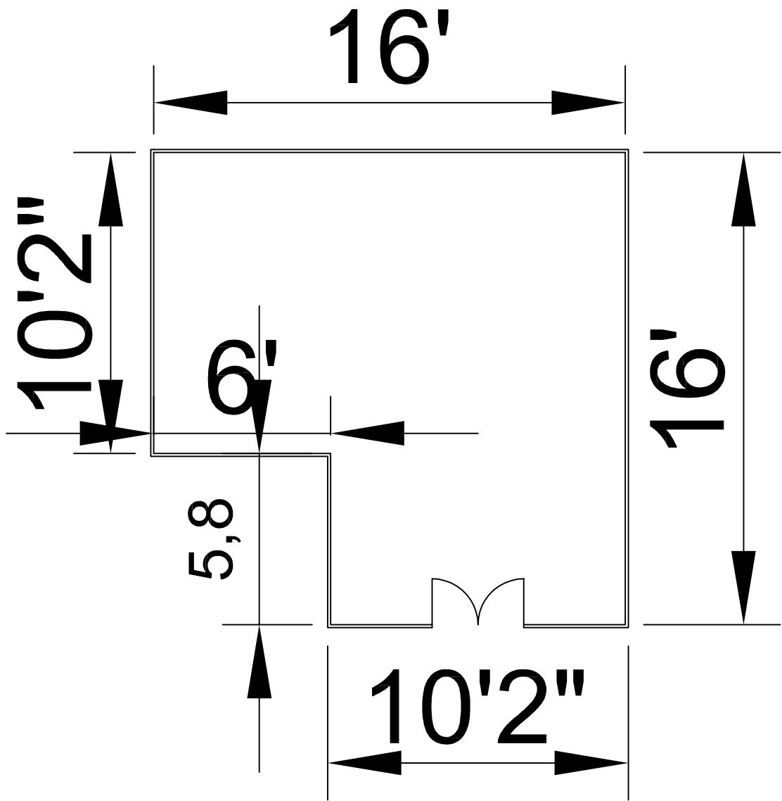
EZCC ROOM DRAWING.
