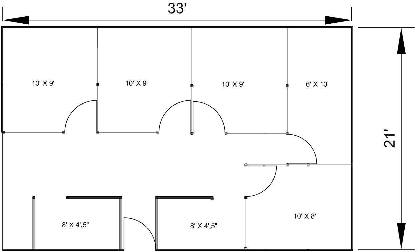
HEIGHT UP TO FALSE CEILING 8' PLAN DRAWING
